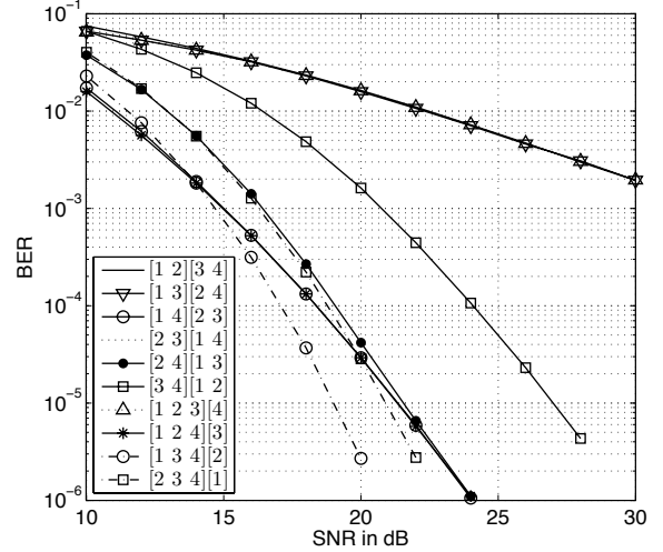
Fig. 4. BER vs. SNR for 4 \times 4 S = 4 , 4-QAM PPMB.
