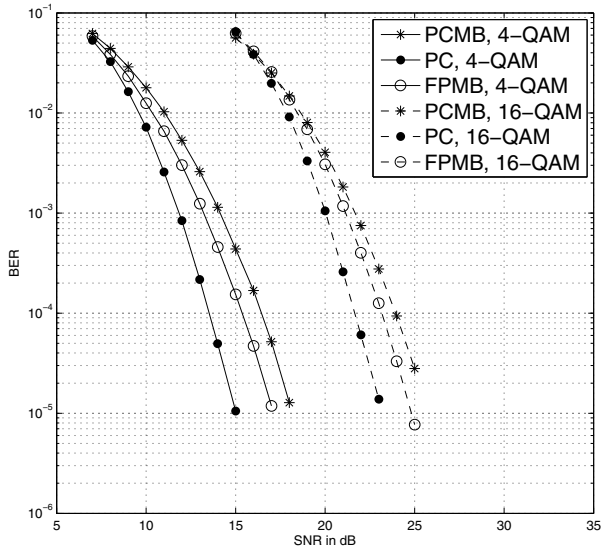
Fig. 3. BER vs. SNR for PCMB, PC and FPMB 4 \times 4 systems.
