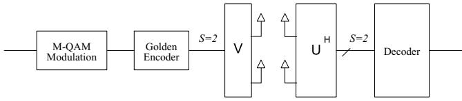
Fig. 1. Structure of GCMB.
